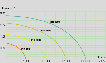
Pumps output vs Max head
